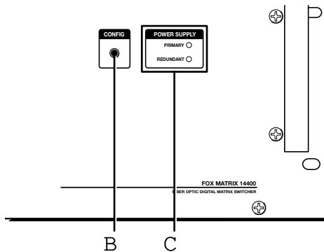
Figure 7. Front Panel Configuration Port, FOX Matrix 14400
