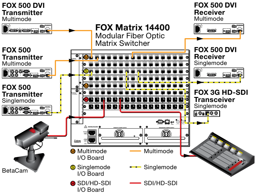
Figure 1. Typical FOX Matrix 14400 application
