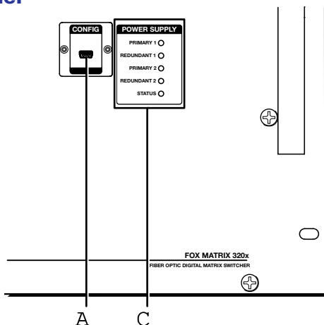
Figure 6. Front Panel Configuration Port, FOX Matrix 320x
