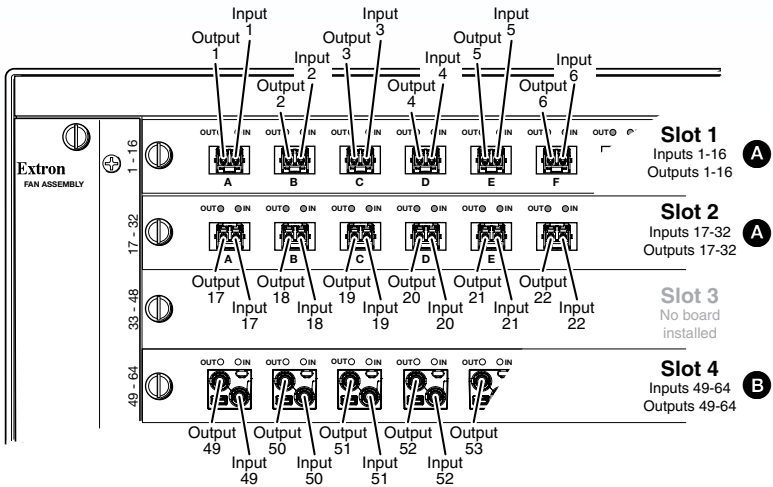
Figure 2. Arrangement of Inputs and Outputs on the I/O Boards
