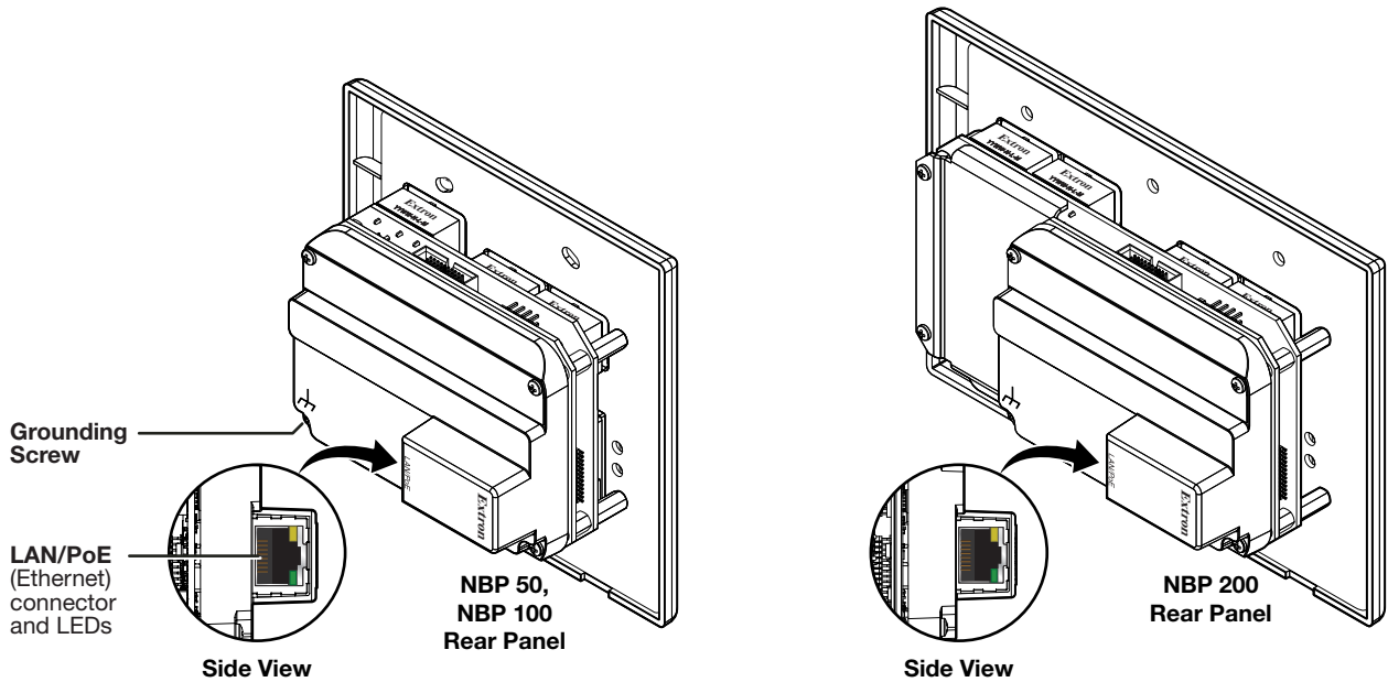
Figure 15. Rear Panel Features — US Gang Models
