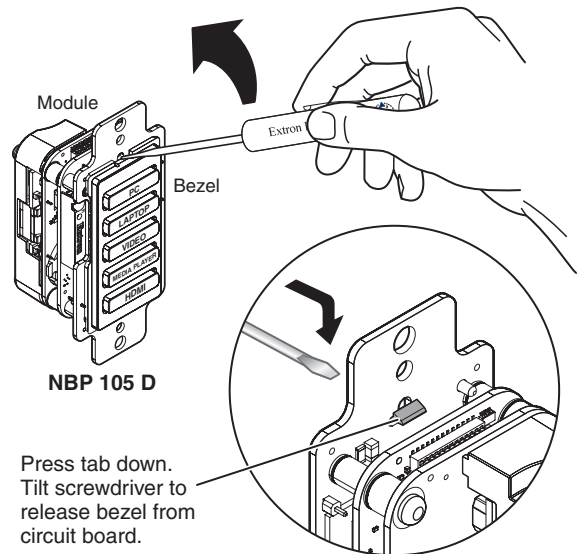
Figure 10. Using a Screwdriver to Release the Bezel Tabs, Rear View
