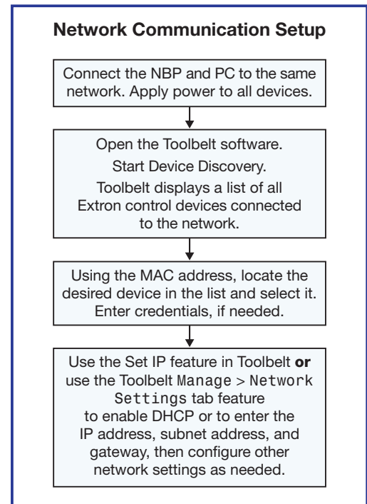
Figure 35. Network Setup
