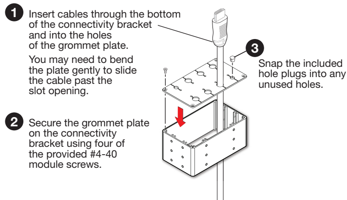
Figure 26. Assembling the Cable Pass-through Module
