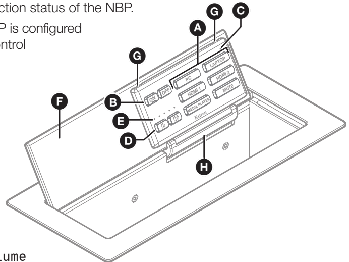
Figure 38. NBP 1200C Front Panel
