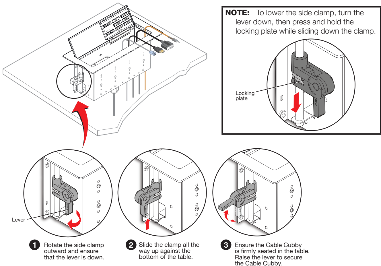
Figure 30. Securing the Cable Cubby Enclosure
