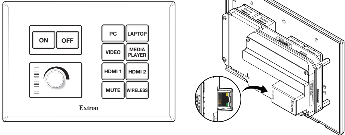
Figure 3. NBP 200 Front (Left) and Rear (Right) Views
