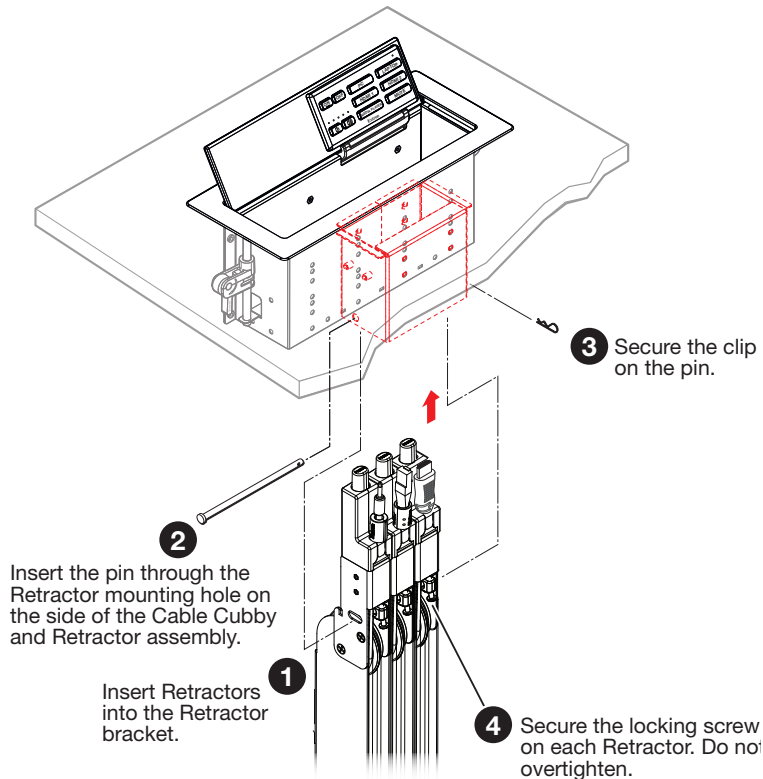
Figure 31. Installing Retractors
