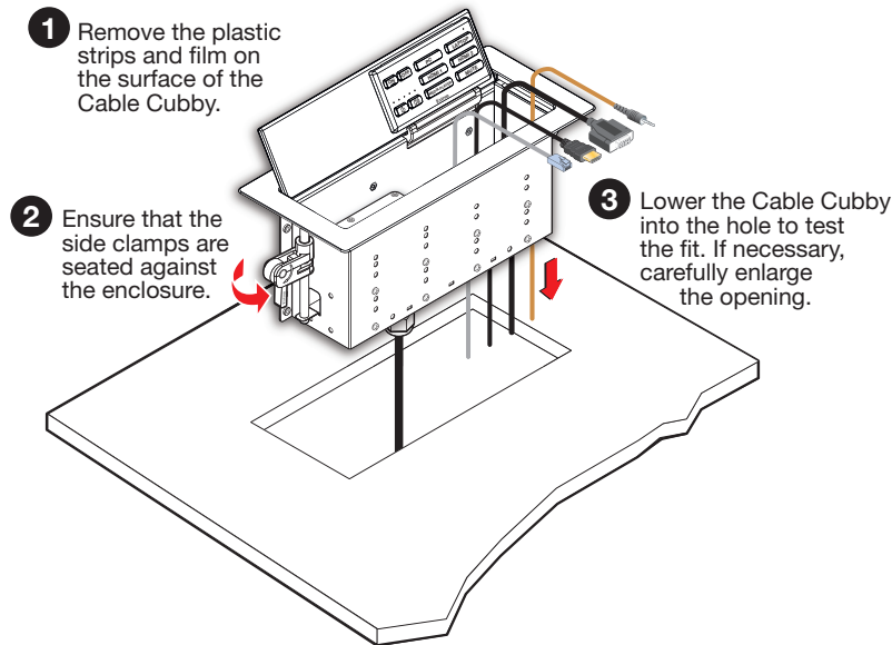
Figure 29. Inserting the NBP 1200C Enclosure into the Table
