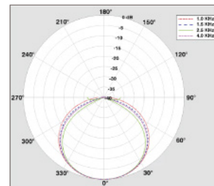
Wide Beam, HPBW = 55 Degrees
