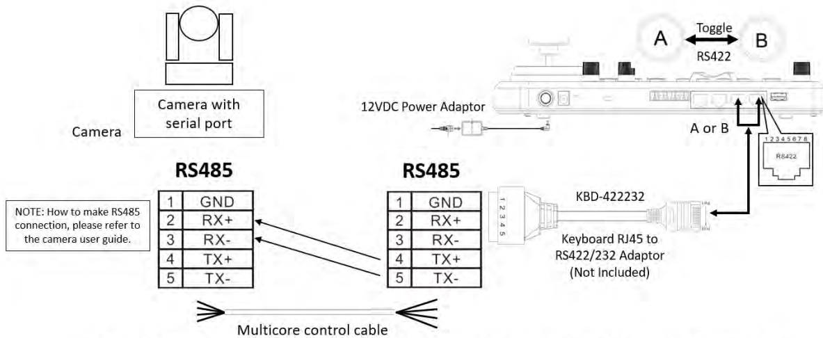
RS485 Connection - Use RJ45-RS422 adapter - Camera with RS485 serial connector
