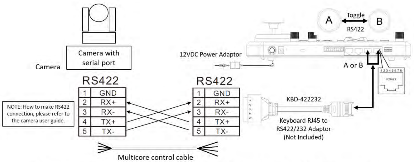
RS422 Connection - Use RJ45-RS422 adaptor - Camera with RS422 serial connector
