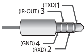
RS-232C (Serial port)
